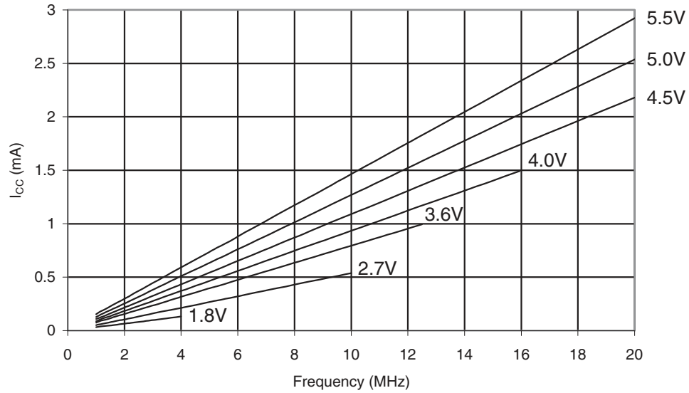
Figure 35-46. ATmega328P Reset Supply Current vs. Frequency (1MHz - 20MHz)
