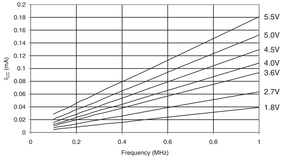
Figure 35-6. ATmega328P: Idle Supply Current vs. Low Frequency (0.1MHz - 1.0MHz)
