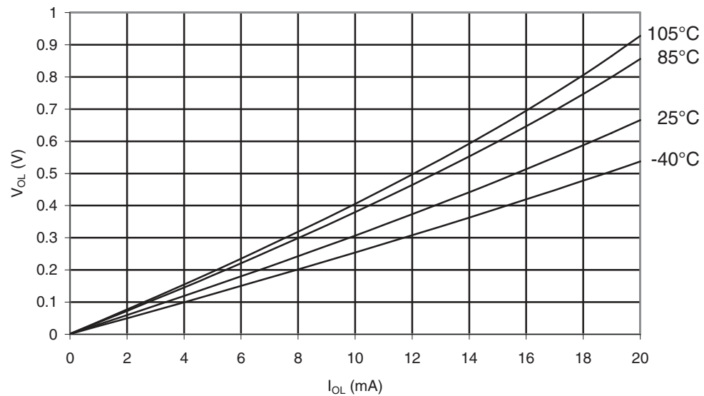
Figure 34-21. ATmega168PA: I/O Pin Output Voltage vs. Sink Current ( V_{CC} = 3V )
