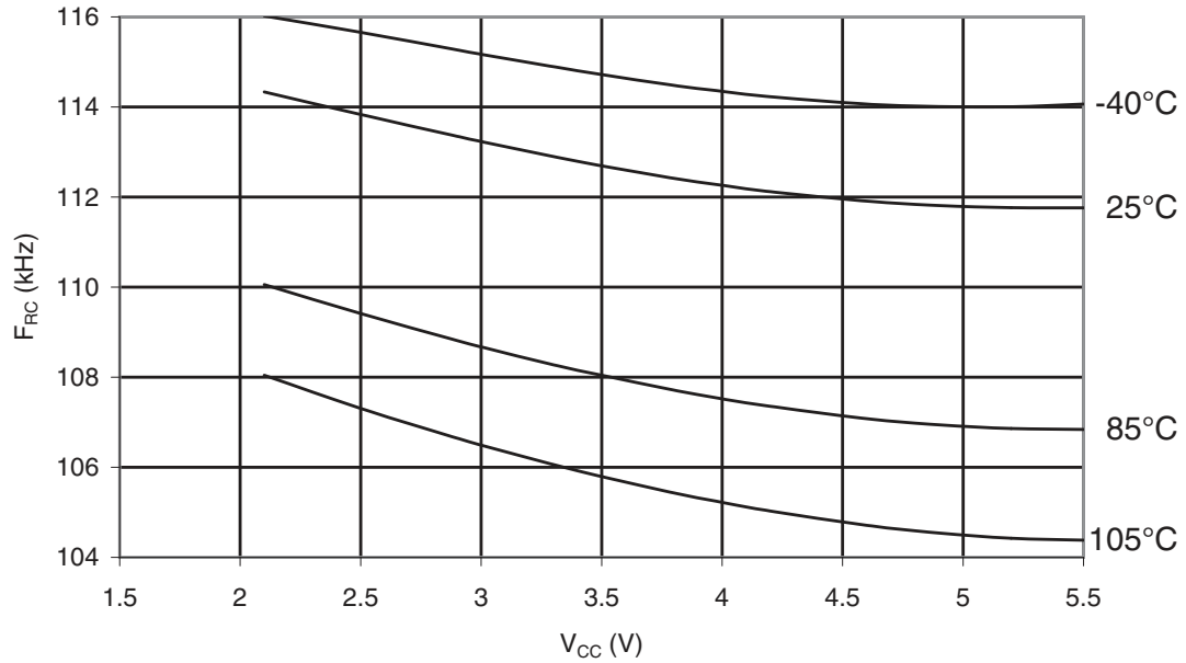
Figure 31-83. ATmega48PA: Watchdog Oscillator Frequency vs. V_{CC}
