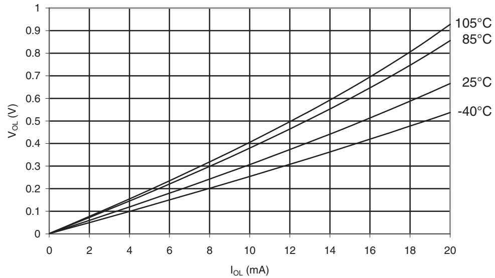
Figure 31-257. ATmega168PA: I/O Pin Output Voltage vs. Sink Current ( V_{CC} = 3V )
