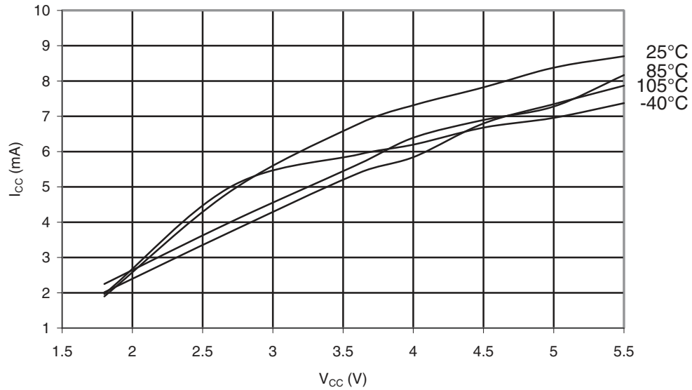
Figure 35-44. ATmega328P: Programming Current vs. V_{CC}
