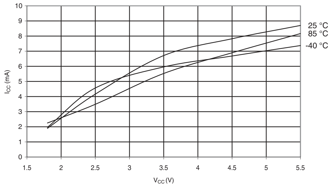
Figure 31-328. ATmega328: Programming Current vs. V_{CC}
