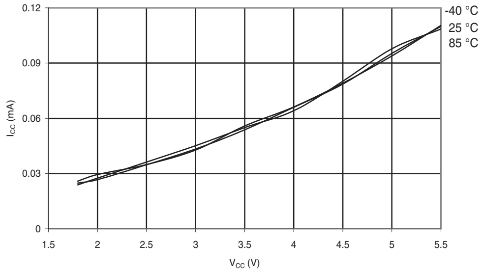
Figure 31-97. ATmega88A: Active Supply Current vs. V_{CC} (Internal RC Oscillator, 128kHz)
