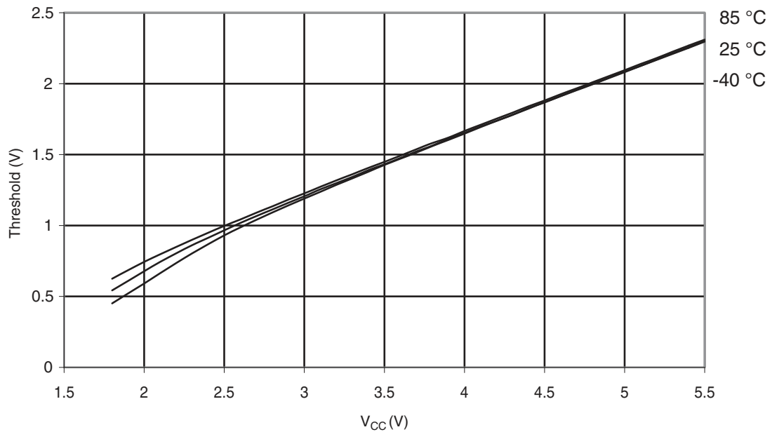
Figure 31-310. ATmega328: I/O Pin Input Threshold Voltage vs. V_{CC} ( V_{IL} , I/O Pin read as '0')
