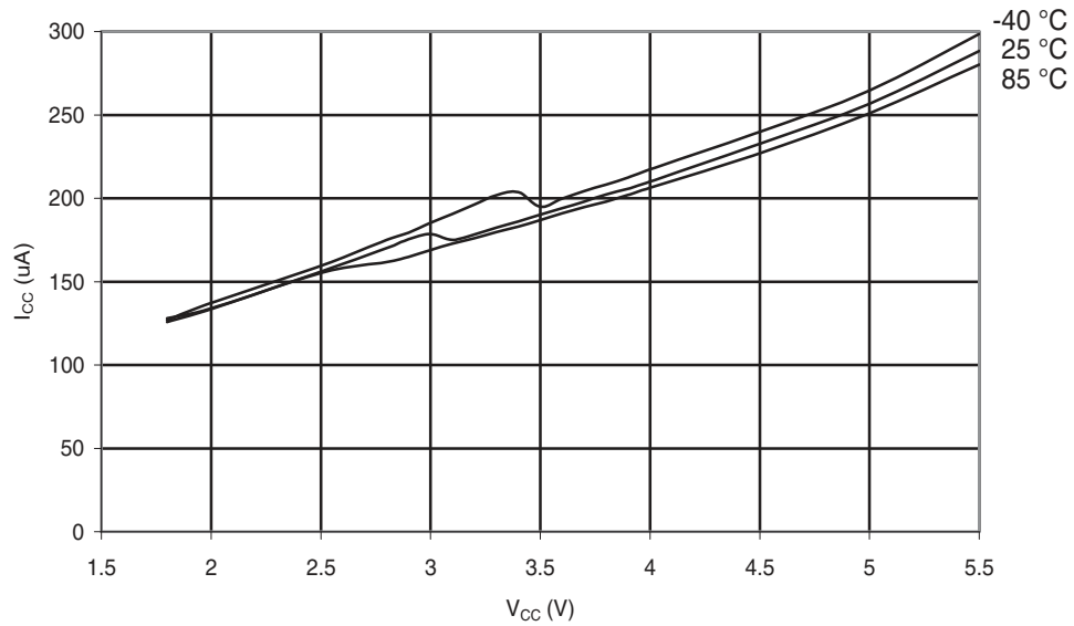
Figure 31-134. ATmega88A: ADC Current vs. V_{CC} (AREF = AV_{CC} )
