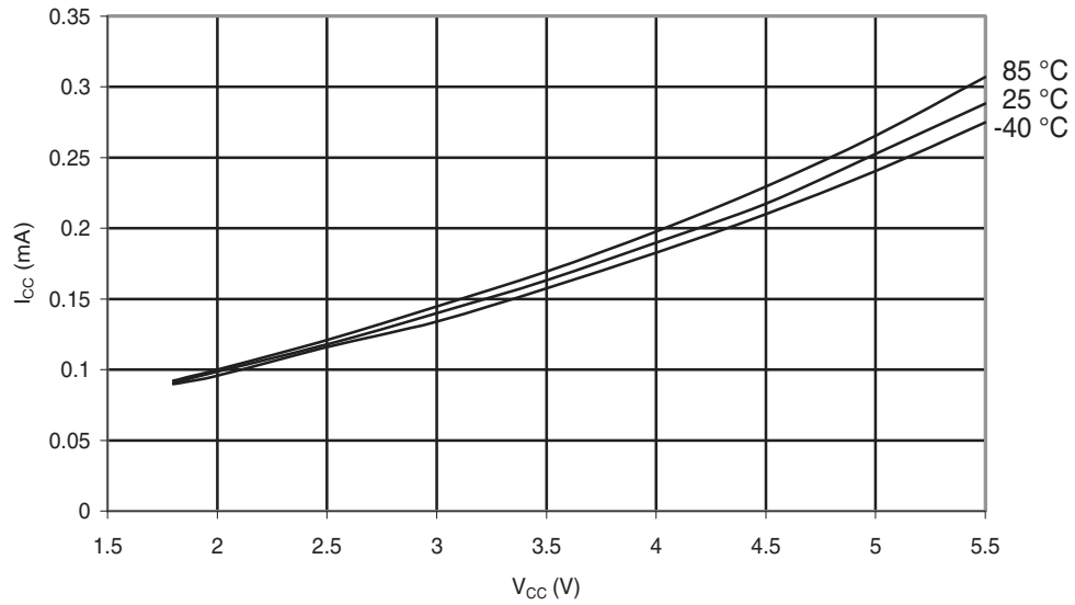
Figure 31-9. ATmega48A: Idle Supply Current vs. V_{CC} (Internal RC Oscillator, 1MHz)
