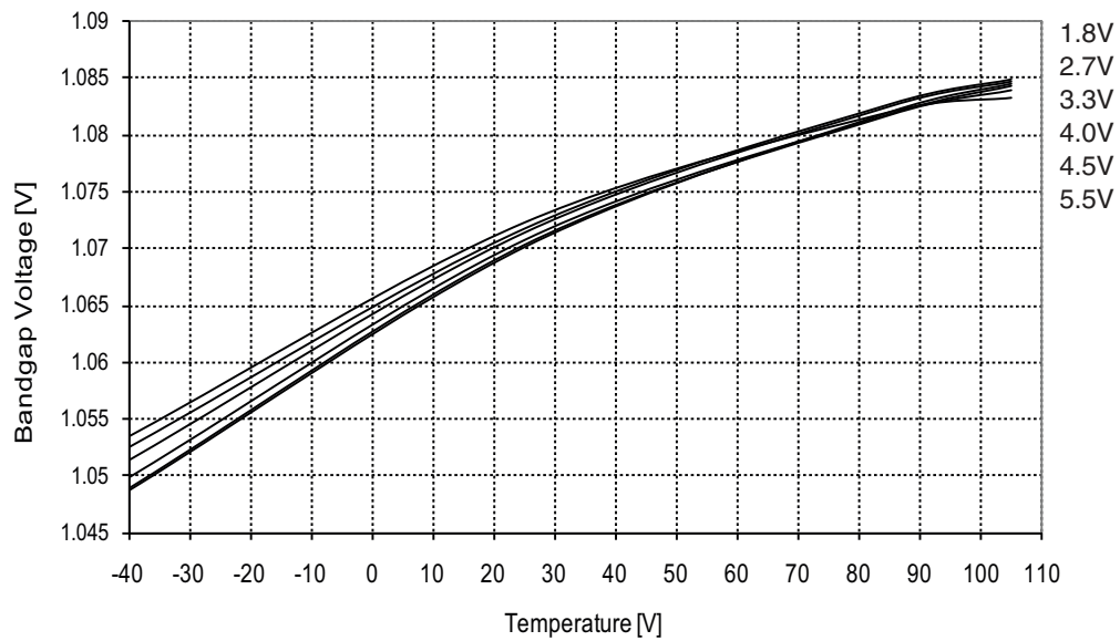
Figure 31-175. ATmega88PA: Calibrated Bandgap Voltage vs. Temperature
