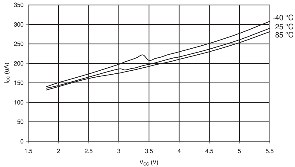
Figure 31-40. ATmega48A: ADC Current vs. V_{CC} (AREF = AV_{CC} )
