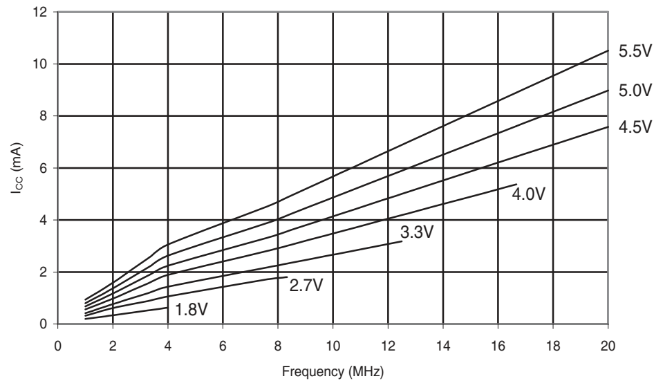
Figure 31-2. ATmega48A: Active Supply Current vs. Frequency (1-20MHz)
