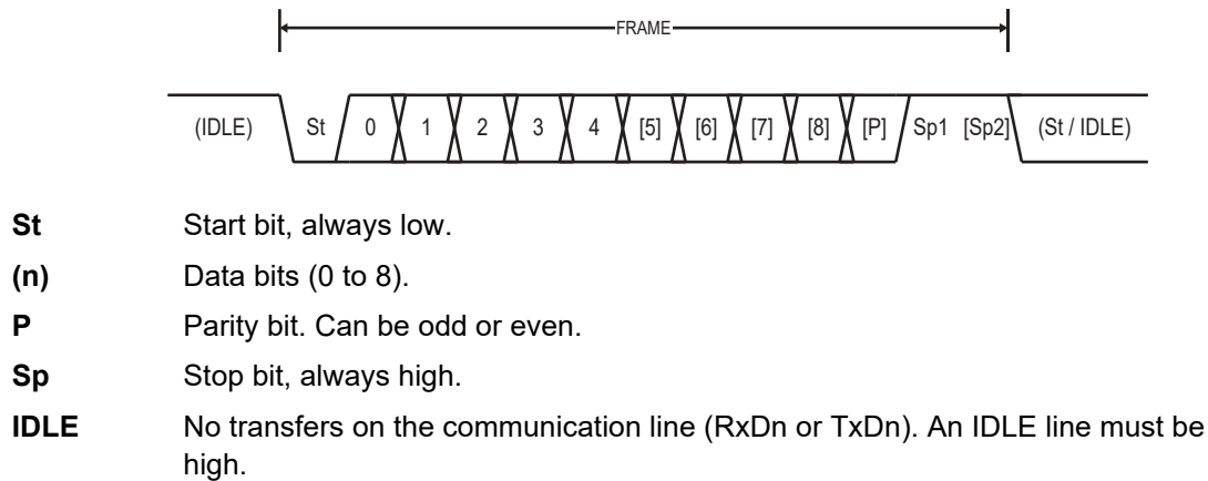
Figure 20-4. Frame Formats
