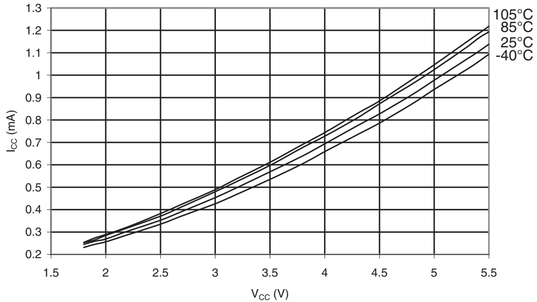
Figure 32-10. ATmega48PA: Idle Supply Current vs. V_{CC} (Internal RC Oscillator, 8MHz)
