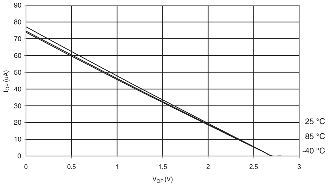
Figure 31-300. ATmega328: I/O Pin Pull-up Resistor Current vs. Input Voltage ( V_{CC} = 2.7\text{ V} )
