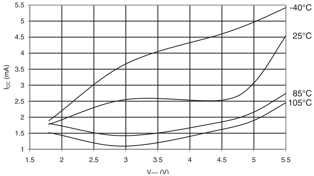
Figure 32-42. ATmega48PA: Programming Current vs. V_{CC}
