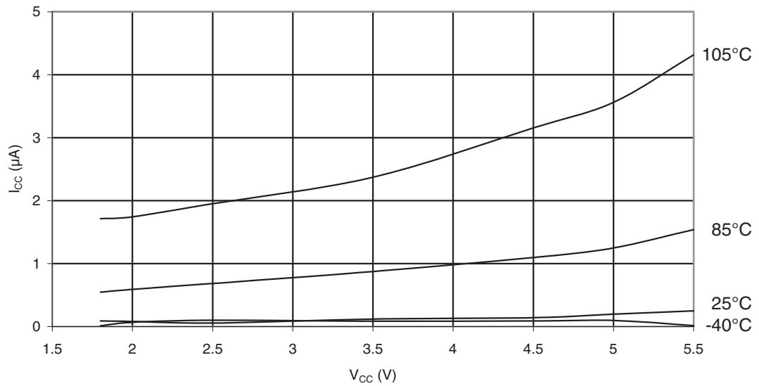
Figure 33-11. ATmega88PA: Power-Down Supply Current vs. V_{CC} (Watchdog Timer Disabled)
