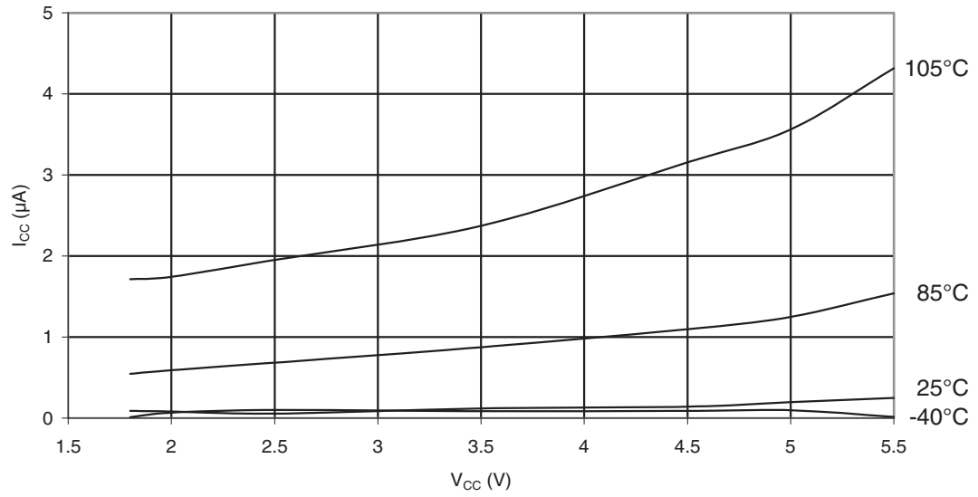
Figure 31-153. ATmega88PA: Power-Down Supply Current vs. V_{CC} (Watchdog Timer Enabled)
