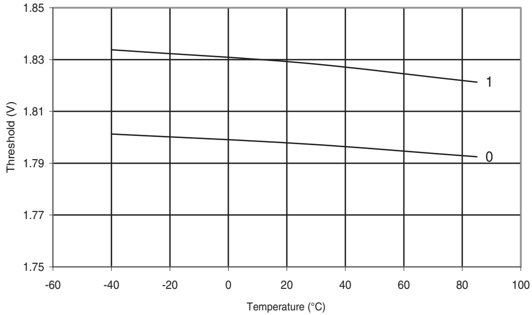
Figure 31-315. ATmega328: BOD Thresholds vs. Temperature (BODLEVEL is 1.8 V)
