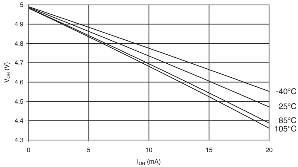
Figure 34-24. ATmega168PA: I/O Pin Output Voltage vs. Source Current ( V_{CC} = 5V )
