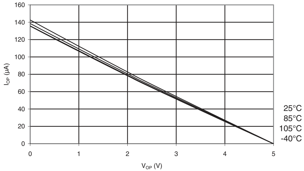
Figure 35-17. ATmega328P: I/O Pin Pull-up Resistor Current vs. Input Voltage ( V_{CC} = 5V )
