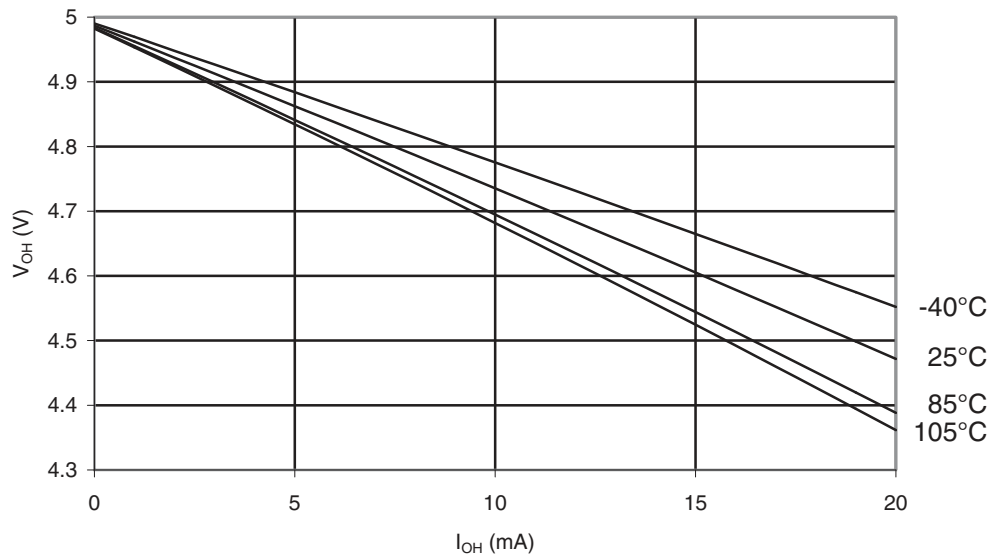
Figure 31-260. ATmega168PA: I/O Pin Output Voltage vs. Source Current ( V_{CC} = 5V )
