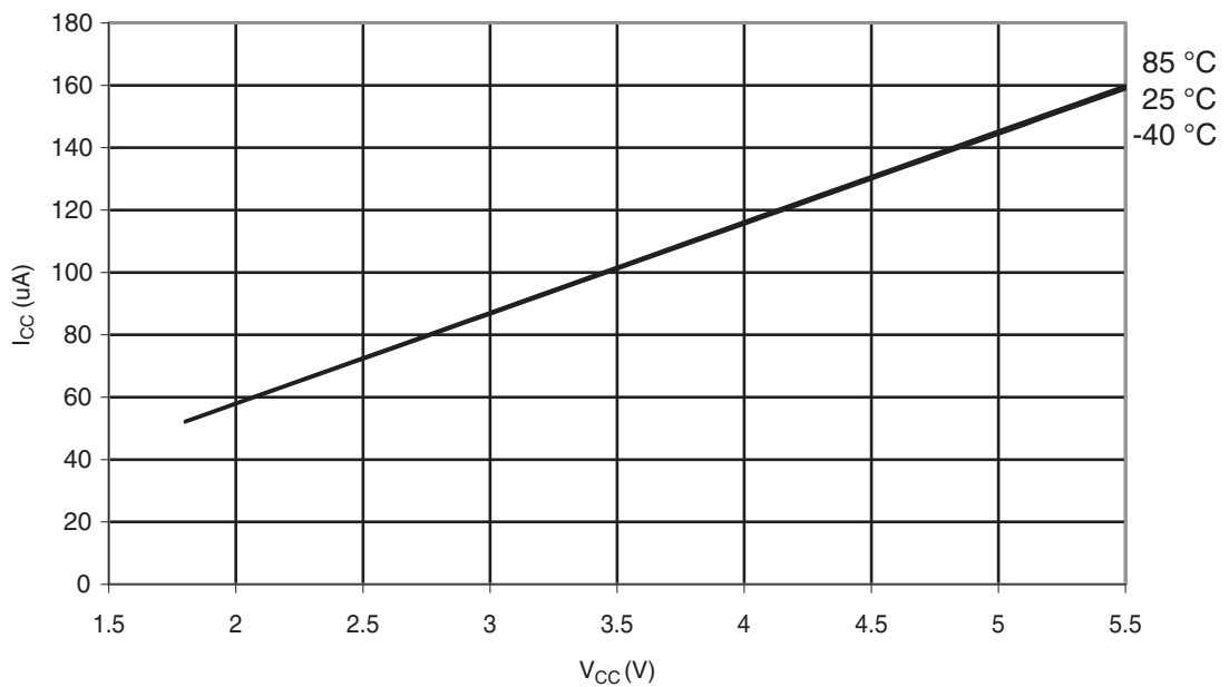
Figure 31-326. ATmega328: AREF External Reference Current vs. V_{CC}
