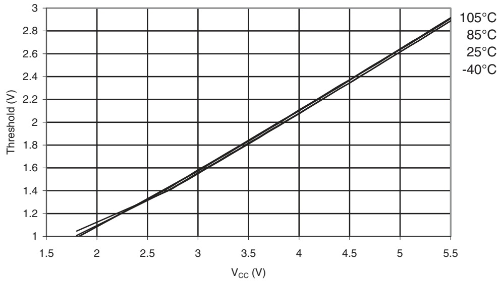
Figure 31-261. ATmega168PA: I/O Pin Input Threshold Voltage vs. V_{CC} ( V_{IH} , I/O Pin read as '1')
