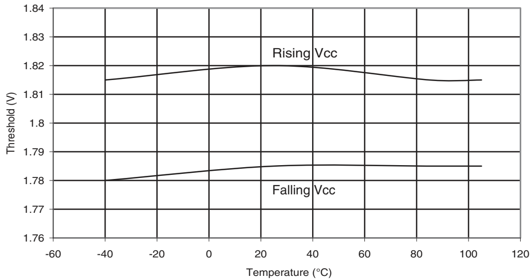
Figure 33-30. ATmega88PA: BOD Thresholds vs. Temperature (BODLEVEL is 1.8V)
