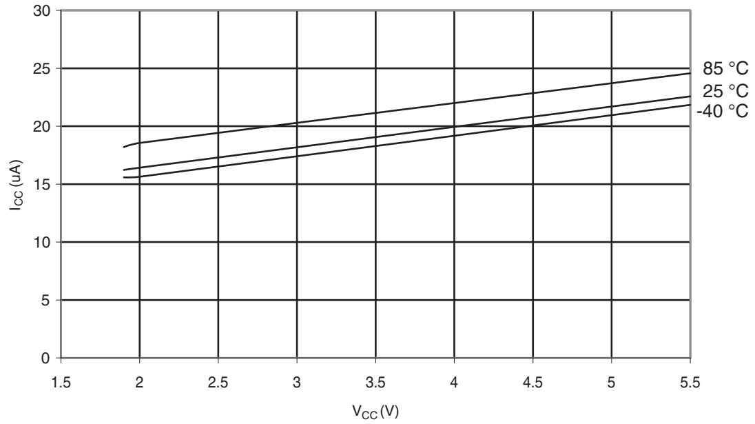
Figure 31-327. ATmega328: Brownout Detector Current vs. V_{CC}
