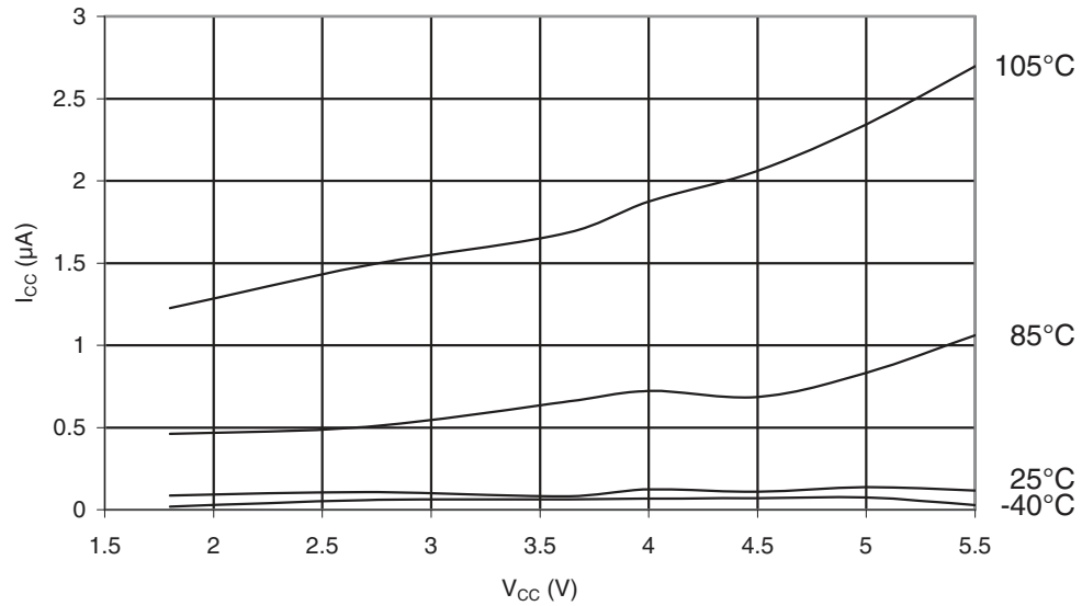
Figure 35-11. ATmega328P: Power-Down Supply Current vs. V_{CC} (Watchdog Timer Disabled)
