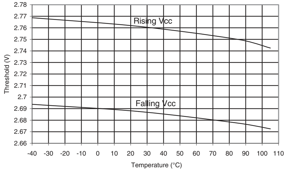
Figure 35-32. ATmega328P: BOD Thresholds vs. Temperature (BODLEVEL is 2.7V)
