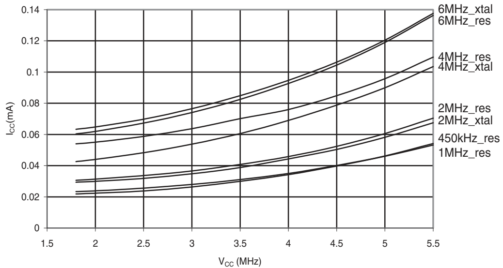
Figure 31-203. ATmega168A: Standby Supply Current vs. V_{CC} (Watchdog Timer Disabled)
