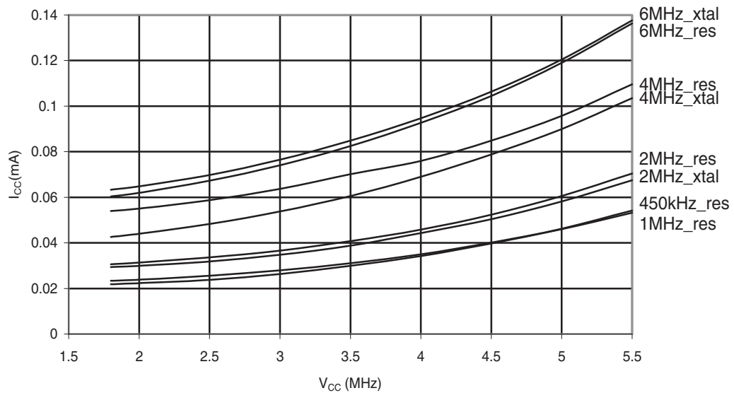
Figure 31-250. ATmega168PA: Standby Supply Current vs. V_{CC} (Watchdog Timer Disabled)
